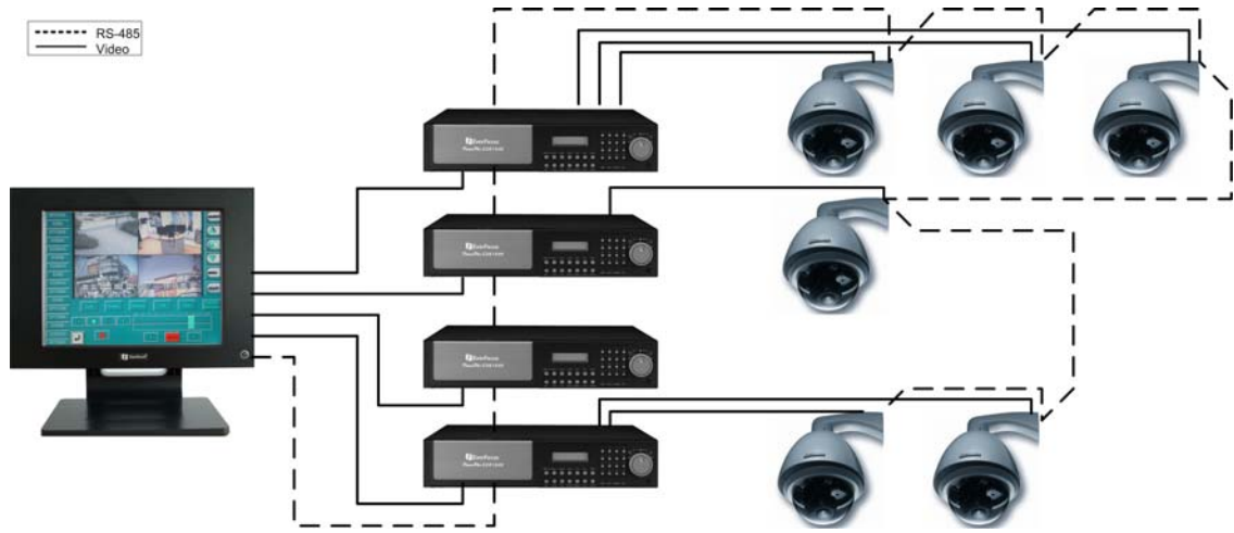
System example with TFT touchscreen control panel ECS 7710 T / cascading I
