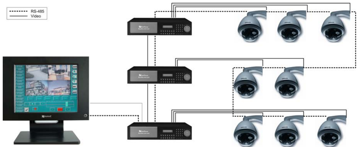
System example with TFT touchscreen control panel ECS 7710 T / cascading II
