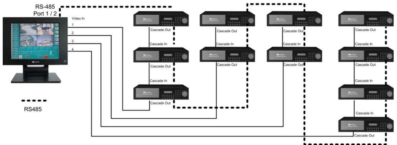
System example with TFT touchscreen control panel ECS 7710 T / cascading II
