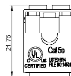
Rear Aspect
