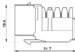
Side Aspect
