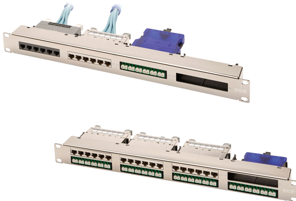
Photography shows 1U 4 Port, 1U 8 Port panels loaded with Copper and Fibre optic modules.
